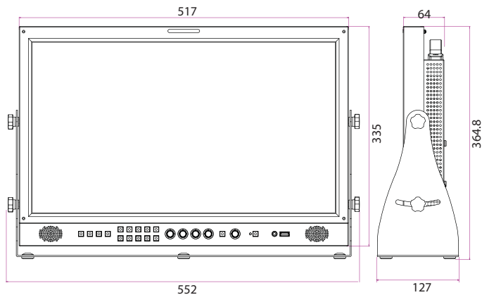
OBM-H 210 Dimensions(mm)
