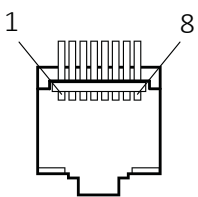
[Pin Assignment]
